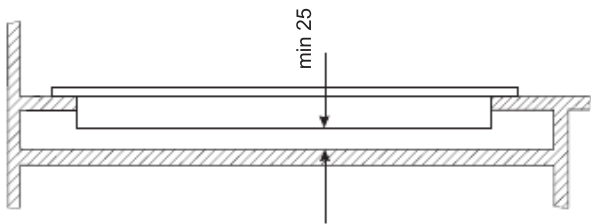
Installing hob in kitchen cabinet worktop.
